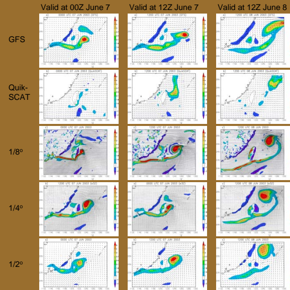
Figure 4: Time evolution of surface wind and vertical vorticity valid at 00 and 12z 7 June and 12z 8 June 2003 from the NCEP GFS analysis, QuikSCAT seawinds, and the 0.125°, 0.25°, and 0.5° runs, respectively from top to bottom.
