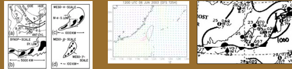
Figure 1 (left): Schematic illustrations of the multi-scale structures of the Mei-Yu frontal zone (from Ohfuchi et al. 2004). Figure 2 (middle): Initial surface winds at 12Z 6 June, 2003. Figure 3 (right): Surface analysis valid at 12Z 8 June, 2003
