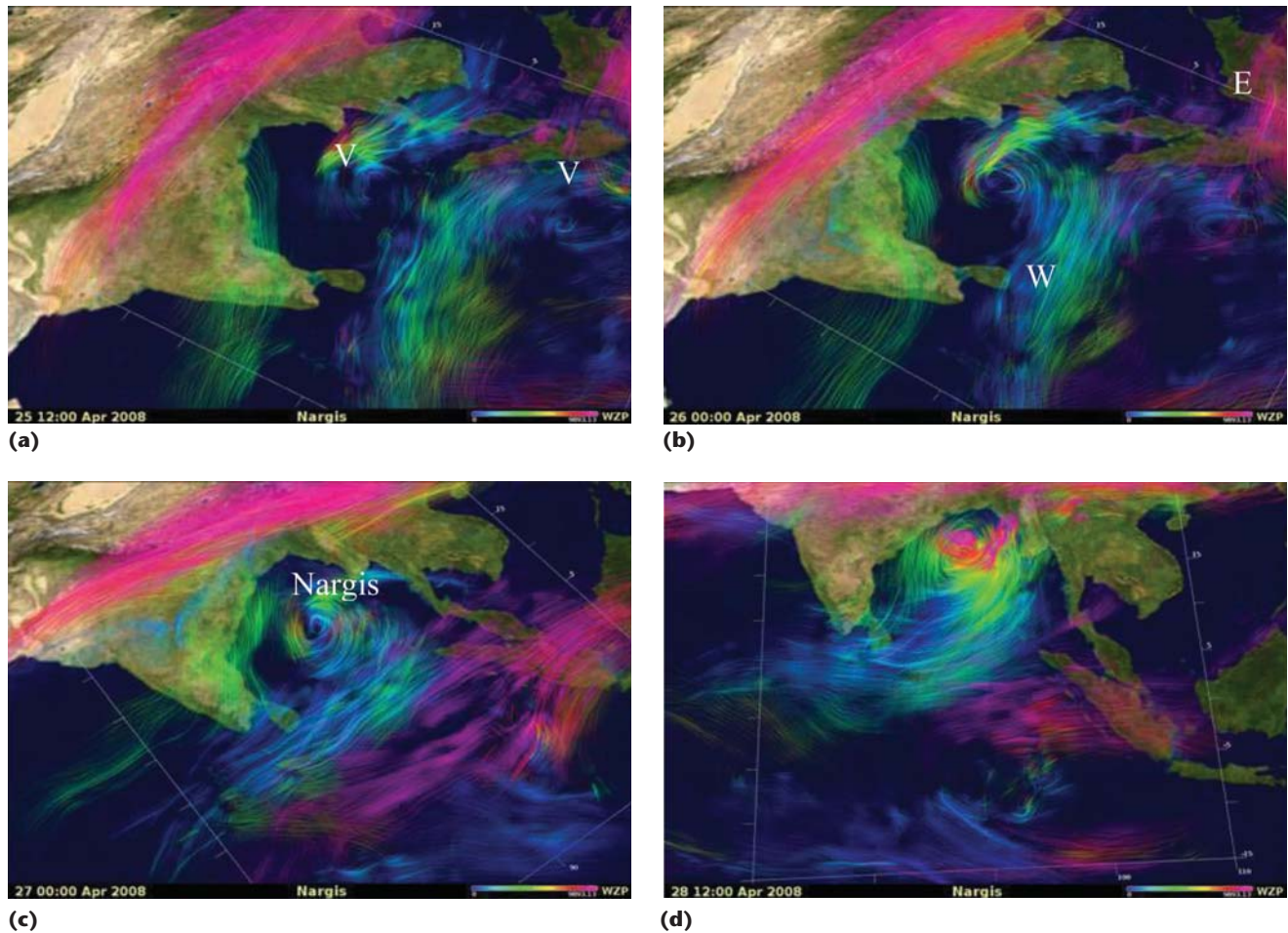
Figure 5. Realistic seven-day simulations of the formation and initial intensification of TC Nargis (2008) initialized at 0000 UTC 22 April 2008, showing streamlines at different levels. Low-level winds are blue and upper-level winds are red. (a) Formation of a pair of low-level vortices (V) at the 84th hour of simulation. (b) Intensification of the northern vortex (left). (c) Formation of Nargis associated with the enhancement of the northern vortex. (d) Intensification of Nargis associated with upper-level outflow and moist processes, indicated by the enhanced upper-level outflow circulation. Approaching upper-level easterly winds (E) increase the vertical wind shear, suppressing the enhancement of the southern vortex (on the right).
